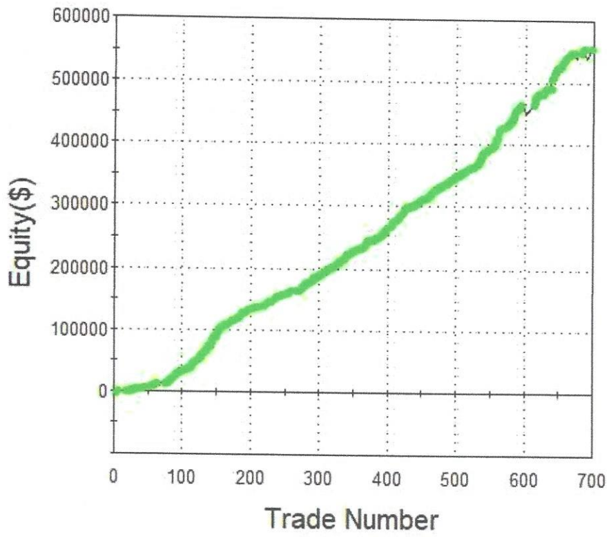
Equity Curve Line - @ES 1440 min.(10/29/2001 17:00 - 10/29/2021 17:00)
